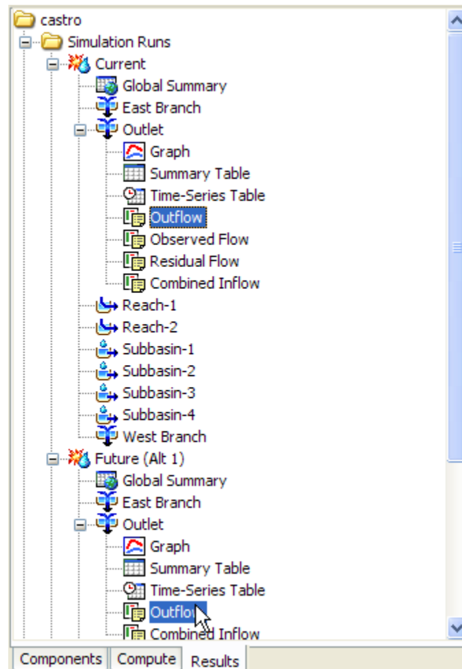
Figure 204. Selecting computed outflow from the same element in two different simulation runs. Other types of time-series data could also be selected.
