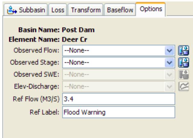
Figure 87. Element component editor for specifying option properties.
