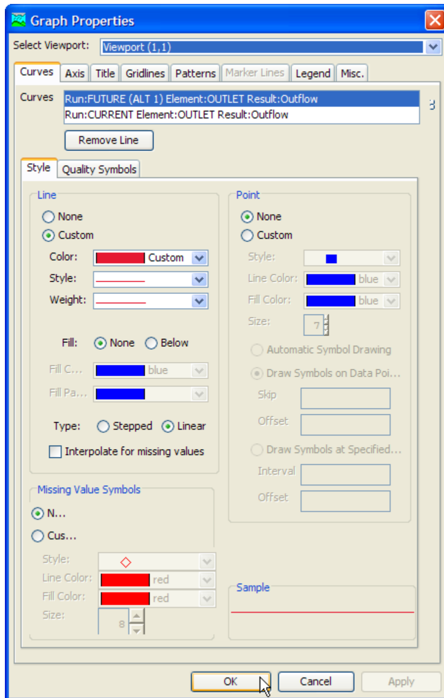
Figure 206. Editing the drawing properties for an element graph.
