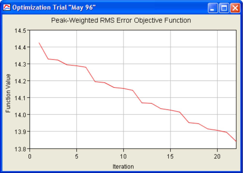
Figure 225. Objective function graph showing the value of the objective function after each iteration in the search.
