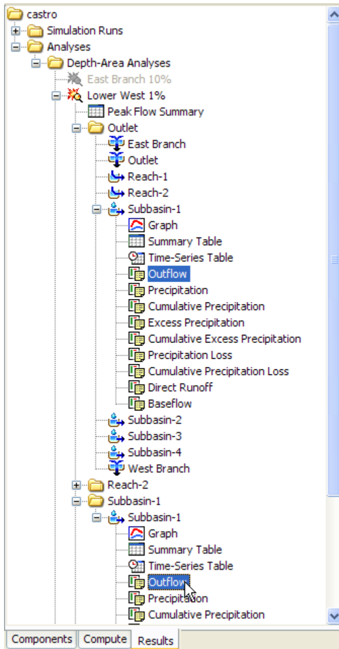
Figure 244. Reviewing the outflow for the same element above two different analysis points in the same depth-area analysis.
