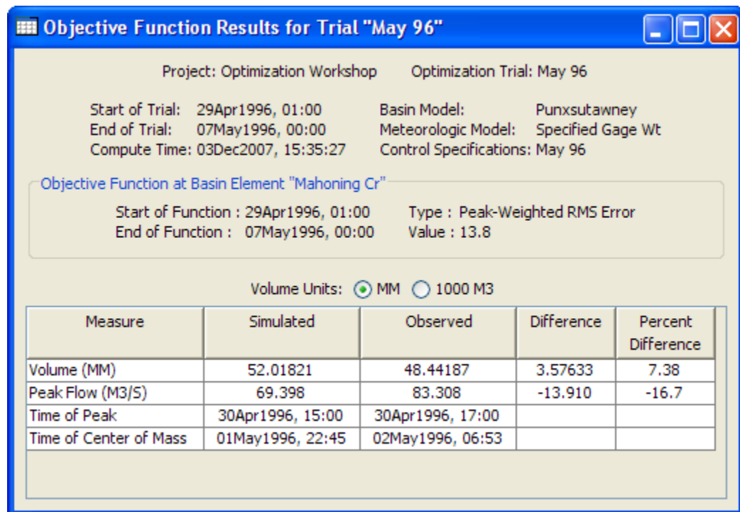
Figure 220. Objective function table for an optimization trial. The table presents statistical results of the computed and observed flow at the optimization location.
