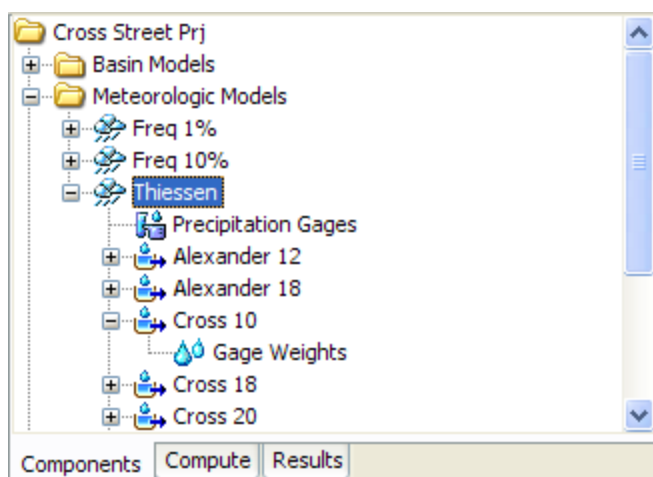
Figure 163. View of a meteorologic model in the Watershed Explorer when the gage weights precipitation method is selected. Options are selected as shown in Figure 162.
