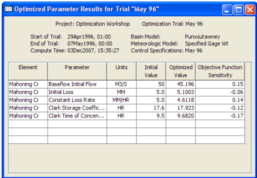
Figure 221. Optimized parameters table for an optimization trial.
