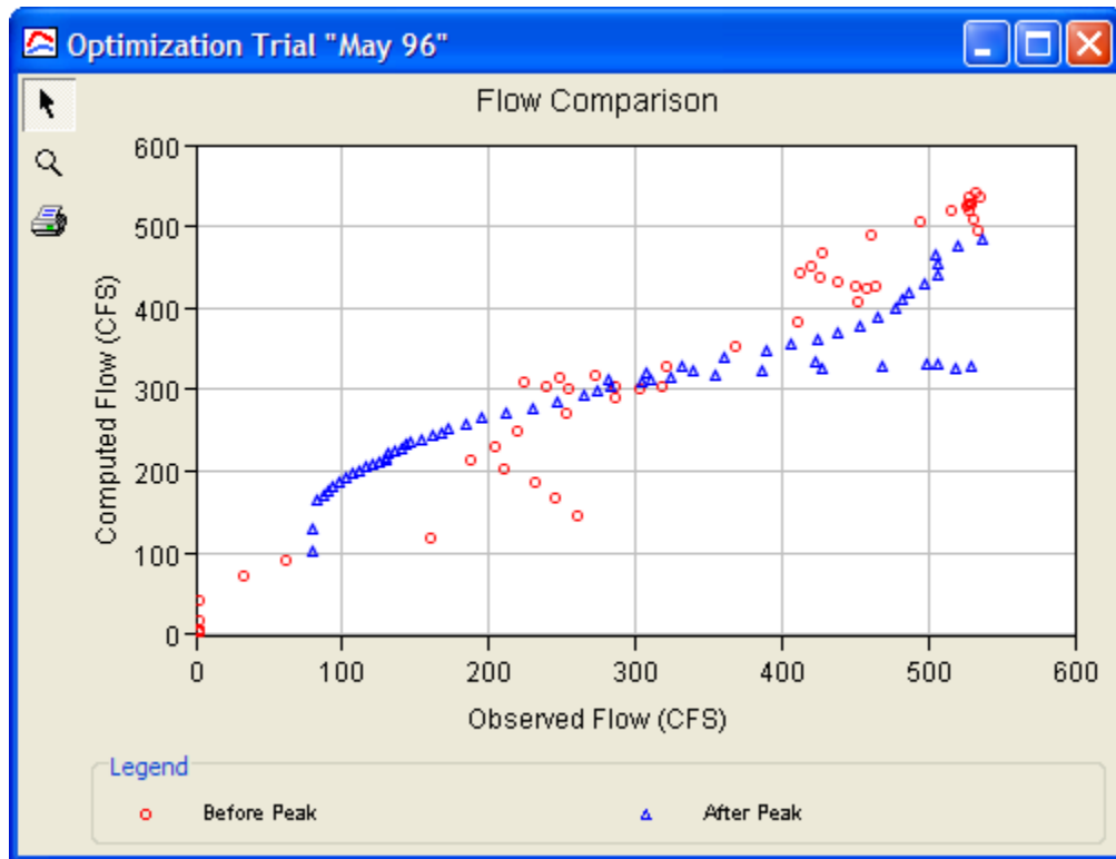
Figure 223. Flow comparison graph showing the computed flow plotted against the observed flow. Different symbols are used for points before and after the observed peak flow.
