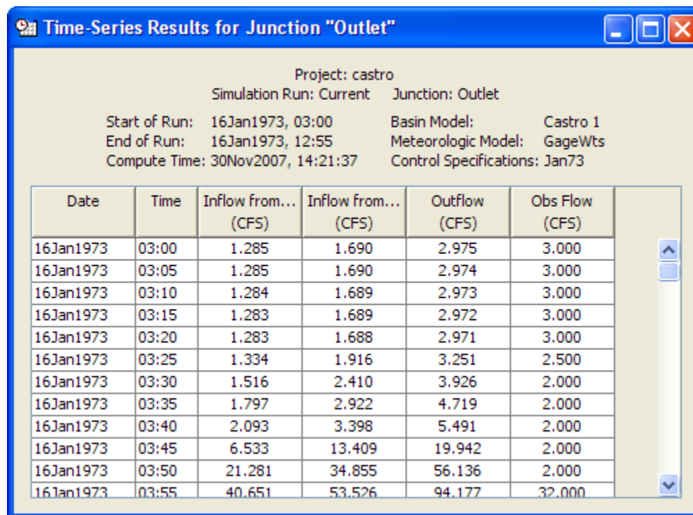
Figure 202. Element time-series table for a junction with observed flow.
