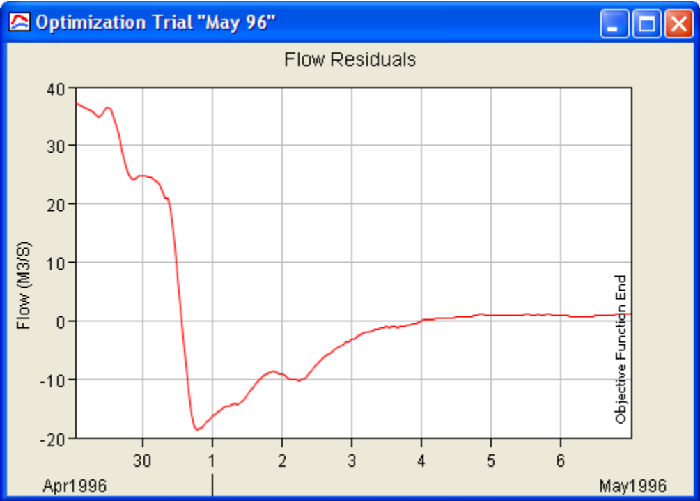
Figure 224. Flow residuals showing the computed minus the observed flow at the optimization location.
