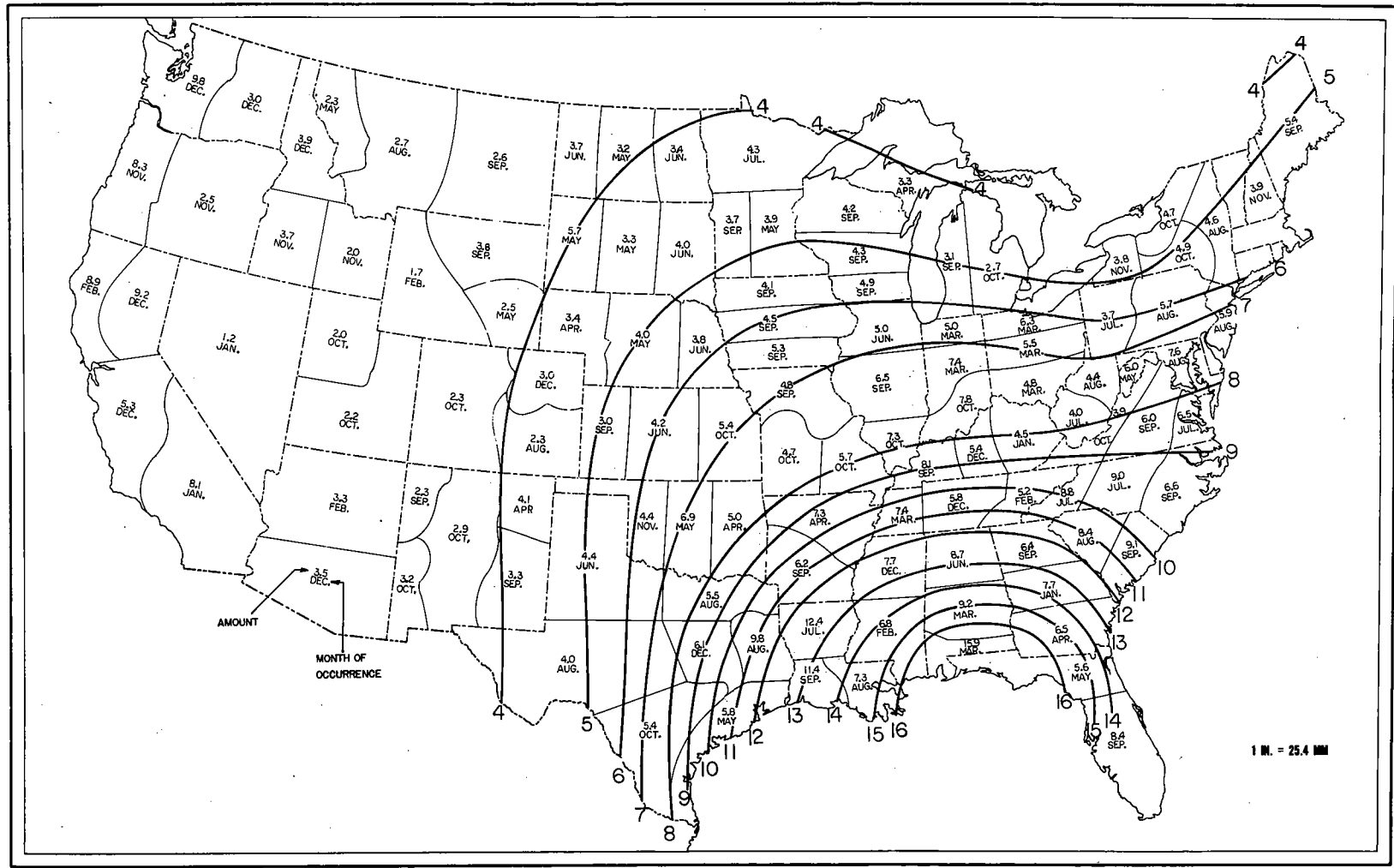
Figure 8.--Envelopment of greatest average weekly precipitation (in.) for State climatic divisions (1906-35).
