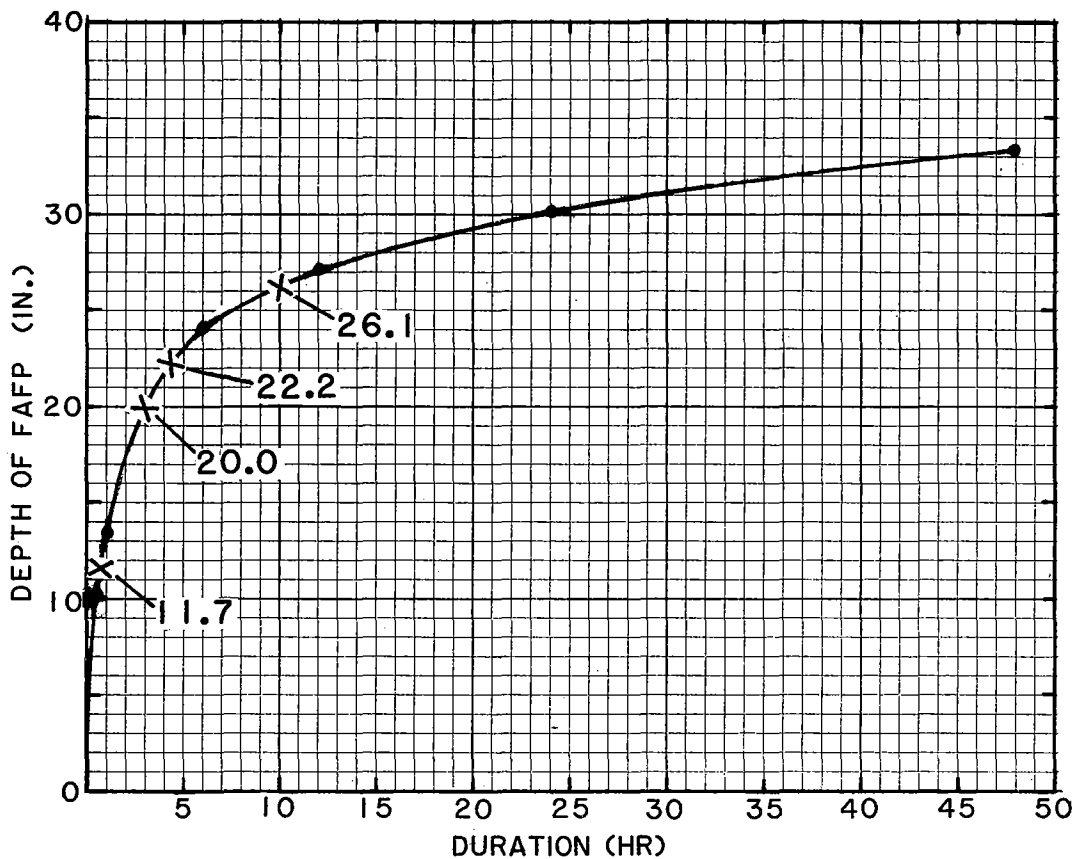
Figure 13.—Depth of FAFP as a function of duration at 42°54'N, 72°57'W near Somerset, VT. The "X's" indicate the interpolated values.
